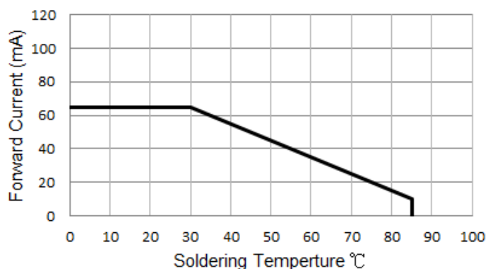
Forward Current VS. Soldering Temperature
